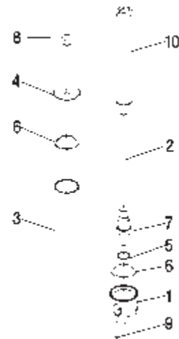
Paint Filter
