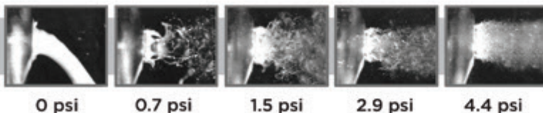
Split Nozzle
