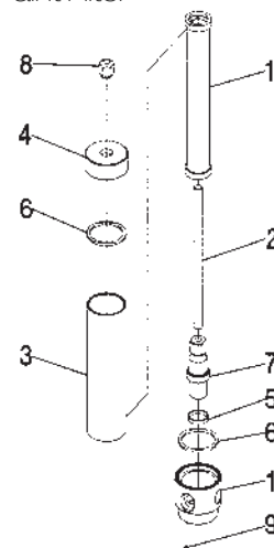
Paint Filter
